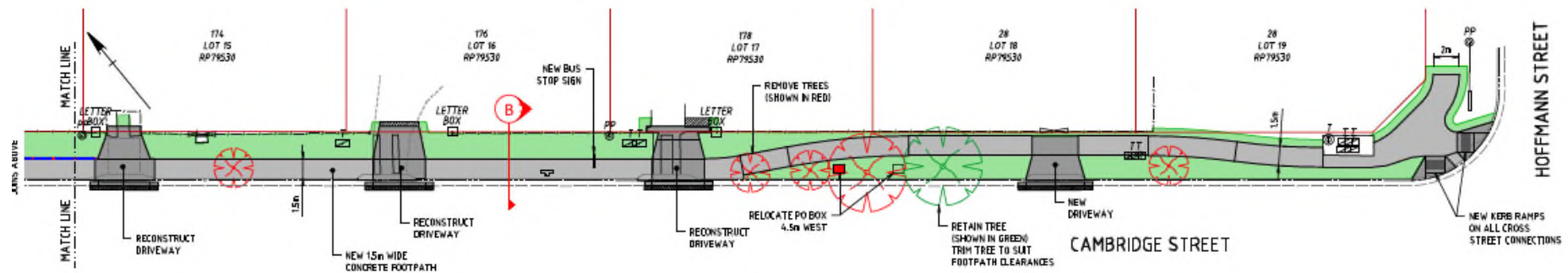
LAYOUT PLAN
