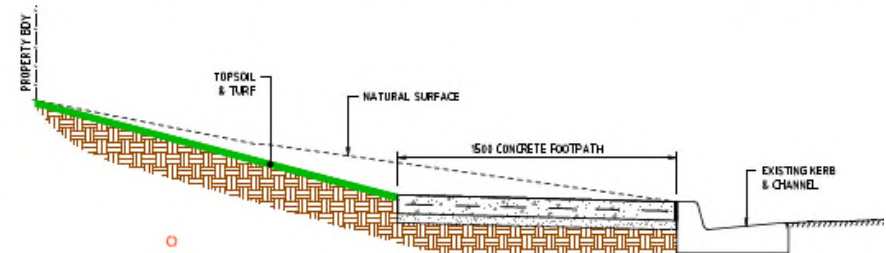
TYPICAL SECTION B - B
