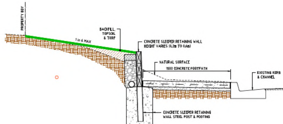
TYPICAL SECTION A - A
